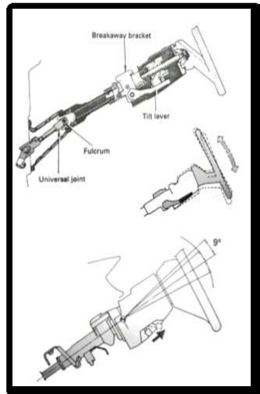
Gambar 3. Tilt Steering "lower fulcrum" dan "upper fulcrum"
