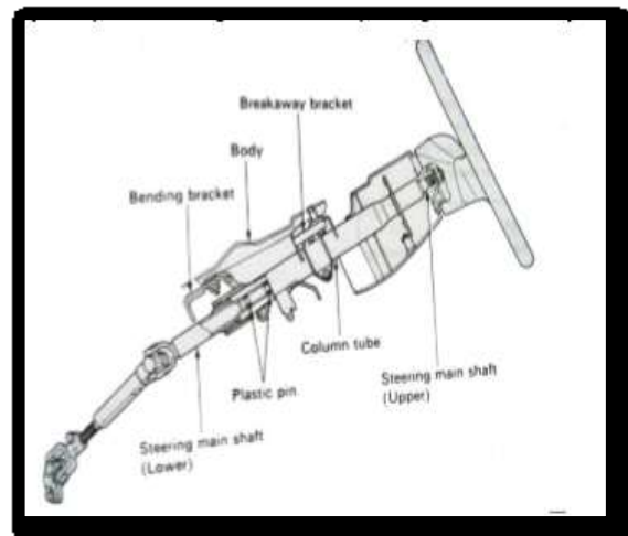
Gambar 2. Steering column
